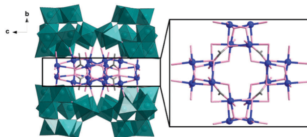
Fig. 1 Representation of the polyanion cluster of 1 (left) and the \{\text{Cu}_{16}\} core in the cluster (right). The \{\text{W}_{11}\} building units are shown as teal polyhedra, Cu as blue sphere, O and C as rose and grey sticks.
