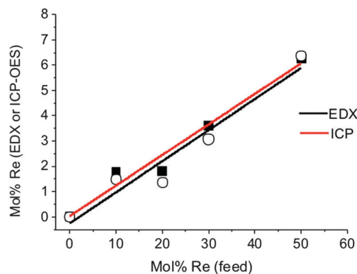
Fig. 5 Plot of mol% Re found in elemental analysis of Mo 1-x Re x S 2 (0 \leq x \leq 0.06) thin films produced by AA-CVD at 475 °C by EDX (■) and ICP-OES (○) spectroscopies as a function of varying mol% of Re in the AA-CVD feed.
