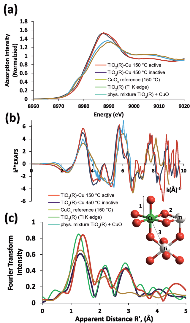
Fig. 4 XAS spectra of photocatalytically active \text{TiO}_2(\text{R}) -Cu (dried at 150 \text{ }^\circ\text{C} ) and inactive \text{TiO}_2(\text{R}) -Cu (calcined at 450 \text{ }^\circ\text{C} ) are compared to the reference data of \text{CuO}_x (prepared by heating), rutile \text{TiO}_2(\text{R}) (Ti K edge), and a physical mixture of \text{TiO}_2(\text{R}) and CuO. Data are presented as XANES (a), EXAFS (b) and Fourier transform of the EXAFS (c). The inset shows a structural model used for fitting.
