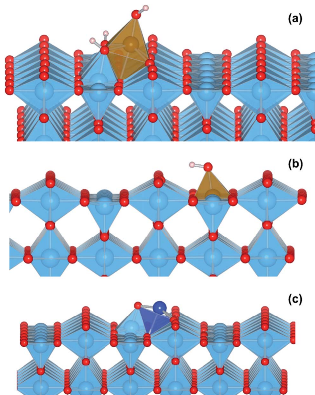
Fig. 6 (a) Final atomic structure of model \text{TiO}_2(\text{R})\text{-Fe} system, red spheres are oxygen atoms, blue spheres are titanium atoms, and brown spheres are iron atoms. (b) Final atomic structure of model \text{TiO}_2(\text{R})\text{-Fe}(\text{V}_{\text{Ti}}) system. (c) Final atomic structure of model \text{TiO}_2(\text{R})\text{-Cu} system, dark blue spheres are copper atoms. Prominent in all structures are the protruding twofold coordinating oxygen atoms of the ideal rutile surface.
