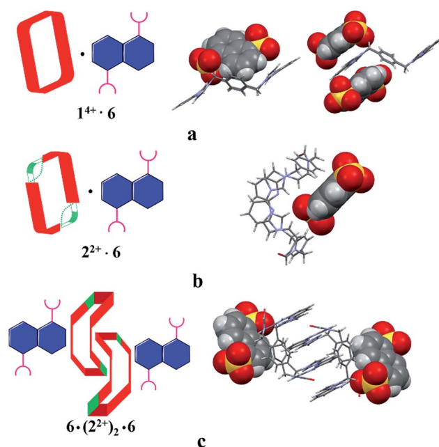
Fig. 5 Schematic views and single crystal X-ray structure of (a) [1 4+ ·6 2 ·6H 2 O], [1 4+ ·6 2 ·14H 2 O], 22c (b) [2 2+ ·6·2.5H 2 O] and (c) 6·(2 2+ ) 2 ·6. Some of the counter ions and solvent molecules have been omitted for clarity.
