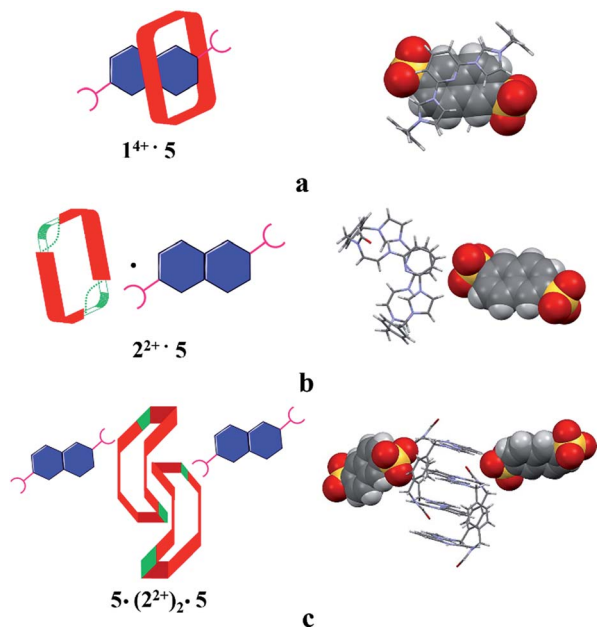
Fig. 4 Schematic views and single crystal X-ray structures of (a) [1 4+ ·5 2 ·7.5H 2 O], 22c (b) [2 2+ ·5·5H 2 O], and (c) 5·(2 2+ ) 2 ·5. Most counter ions and solvent molecules have been omitted for clarity.
