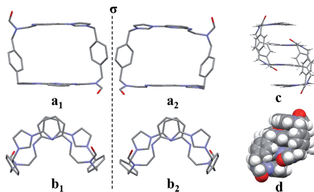
Fig. 2 Top ( a_1 and a_2 ) and side ( b_1 and b_2 ) views of the single crystal X-ray structure of [2^{2+} \cdot 2PF_6^- \cdot CH_3CN \cdot H_2O] showing the enantiomeric pair present in the crystal. Stick (c) and space-filling (d) views of these clip-like enantiomeric pairs. Counter ions and solvent molecules have been omitted for clarity.
