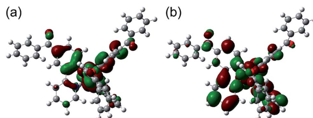
Fig. 4 Optimized geometry structure and electron configurations of (a) HOMO and (b) LUMO for Ir-1c.
