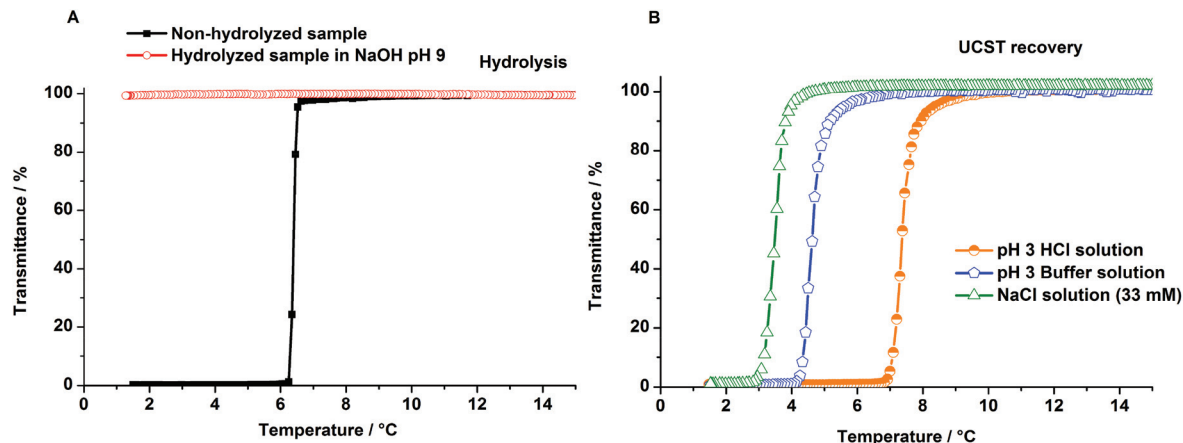
Fig. 4 (A) Hydrolysis of poly(AAm 87 -co-AN 12 ) in NaOH at RT (10 h). (B) Recovery of the thermo-responsive behavior of a hydrolyzed sample of poly(AAm 87 -co-AN 12 ) in NaOH with solutions of pH 3 (buffer and HCl) and with aqueous solutions with NaCl as the chaotropic agent (33 mM).
