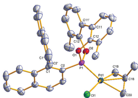
Fig. 4 Molecular structure of ( S )- 7a . Hydrogen atoms have been omitted for clarity. Selected average bond distances (Å) and angles (°): Pd1–P1 2.2368(11), Pd1–Cl1 2.3739(11), Pd1–C18 2.152(4), Pd1–C19 2.095(4), Pd1–C20 2.206(4), P1–C2 1.804(4), P1–O1 1.610(3), P1–O2 1.622(3), C11–C11' 1.485(6); P1–Pd1–Cl1 94.59(4), P1–Pd1–C19 96.50(15), P1–Pd1–C20 162.95(15), C19–Pd1–C20 66.8(2), C19–C18–C20 117.4(5), C2–C1–C1'–C2' –81.9(6), C12–C11–C11'–C12' –46.0(7).
