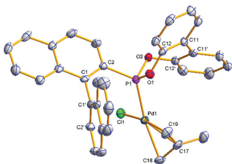
Fig. 3 Molecular structure of ( S )- 6a . Hydrogen atoms have been omitted for clarity. Selected average bond distances (Å) and angles (°): Pd1–P1 2.2478(10), Pd1–Cl1 2.3583(9), Pd1–C17 2.162(4), Pd1–C18 2.195(4), Pd1–C19 2.096(4), P1–C2 1.815(4), P1–O1 1.619(3), P1–O2 1.610(3), C11–C11' 1.477(5); P1–Pd1–Cl1 91.55(4), P1–Pd1–C18 165.51(11), P1–Pd1–C19 98.27(13), C18–Pd1–C19 67.46(16), C18–C17–C19 114.6(4), C2–C1–C1'–C2' –80.8(5), C12–C11–C11'–C12' 42.3(6).
