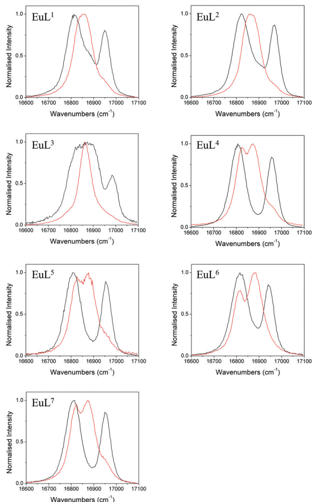
Fig. 5 Normalised emission bands for the ^5D_0 – ^7F_1 transitions of \text{EuL}^{1-7} in the absence (black) and presence (red) of an excess of sodium fluoride (exit slit = 0.2 nm).
