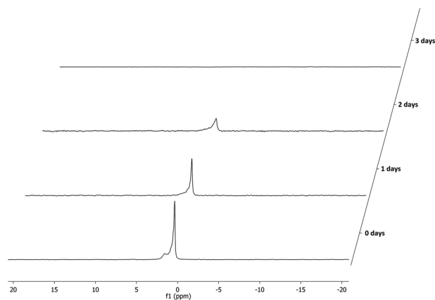
Fig. 3 Hydrolysis of representative supported phosphine–borane sulfate 3a\text{-BH}_3 monitored by ^7\text{Li} NMR spectroscopy.
