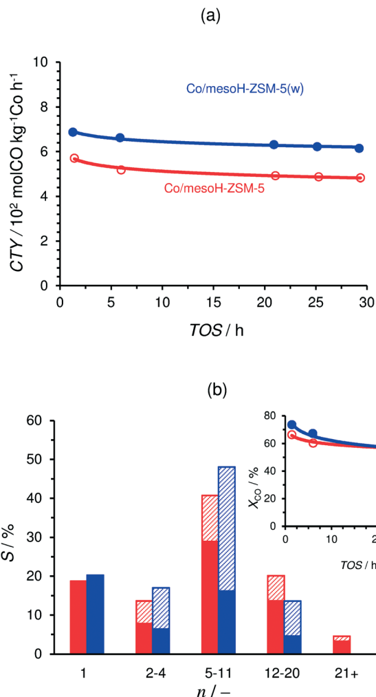
Fig. 8 Time-on-stream (TOS) evolution of the cobalt-time-yield (CTY) during FTS where \text{GHSV} = 12.0 \text{ m}_{\text{STP}}^3 \text{ kg}_{\text{cat}}^{-1} \text{ h}^{-1} (a). Carbon selectivity of the FTS products after 20 h on-stream under iso-conversion conditions (as depicted in the inset) where \text{GHSV} = 12.0 \text{ m}_{\text{STP}}^3 \text{ kg}_{\text{cat}}^{-1} \text{ h}^{-1} for Co/mesoH-ZSM-5 and 24 for Co/mesoH-ZSM-5(w) (b); in each carbon number group from left to right: Co/mesoH-ZSM-5 and Co/mesoH-ZSM-5(w); ■: n -paraffins, ///: sum of isoparaffins and olefins. Experiments were performed at 513 K, 15 bar, \text{H}_2/\text{CO} = 2 .
