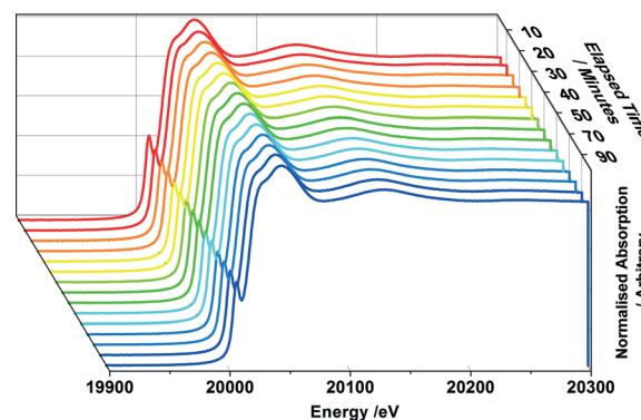
Fig. 7 XANES data over a 90 minute period for 6 ML MoO x /Fe 2 O 3 when reacted isothermally at 250 °C under a continuous flow of MeOH/O 2 . XAFS data was collected continuously using 1 minute scans, whilst Mass Spectrometer data was recorded simultaneously, to ensure a reaction was occurring.
