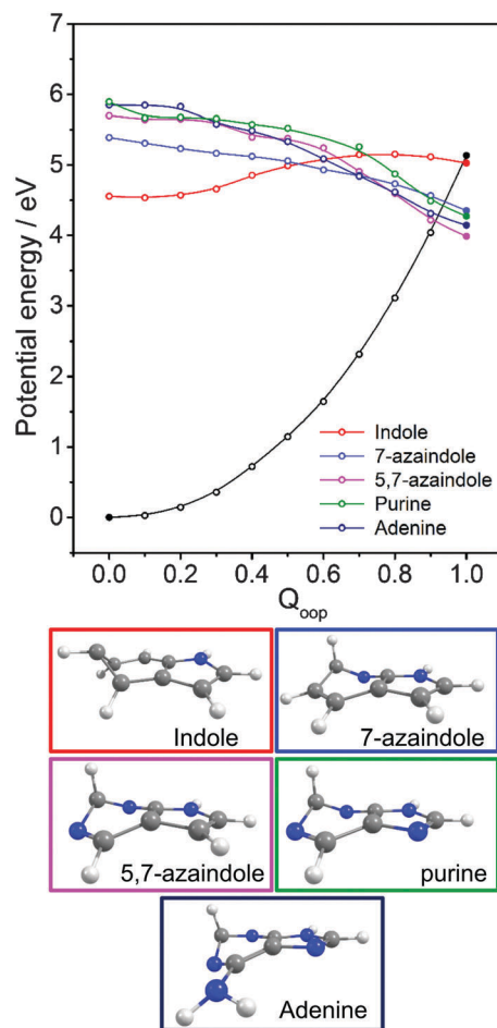
Fig. 13 Overlaid diabatic PECs along Q_{oop} for the 1\pi\pi^* state that correlates with the 1\pi\pi^*/S_0 MECI in indole, 7-azaindole, 5,7-azaindole, purine and A. The filled points show the energies of the optimised critical structures (i.e. the S_0 state minimum and the S_0/1\pi\pi^* MECI) and, for clarity, only the S_0 PEC calculated for indole is shown (open black points). The optimised geometry at each MECI is shown below.
