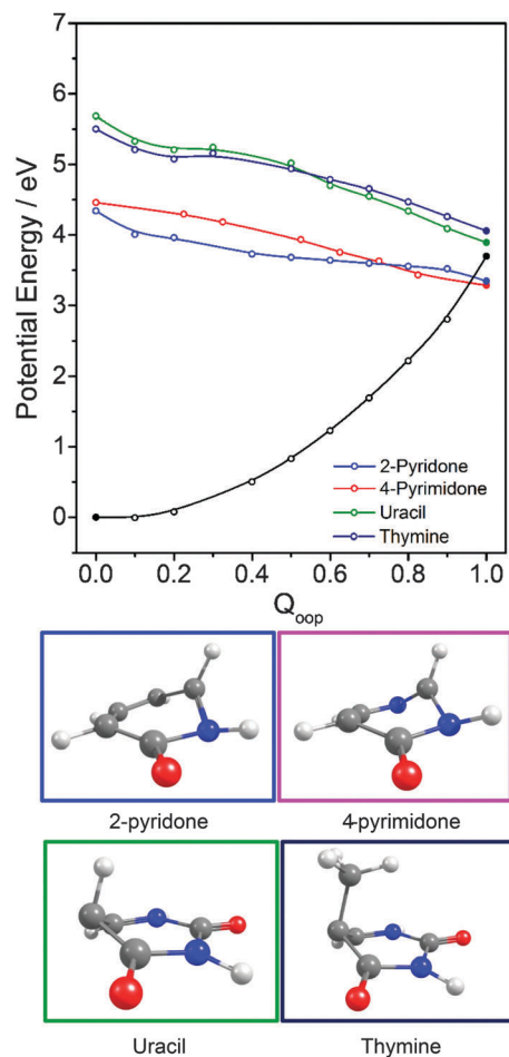
Fig. 11 Overlaid PECs along Q_{\text{oop}} for the 1^1\pi\pi^*/S_0 MECI and respective 1^1\pi\pi^*/S_0 MECIs for 2-pyridone, 4-pyrimidone, U and T along with the calculated S_0 PEC for 2-pyridone. The filled points show the energies of the optimised critical structures ( i.e. the S_0 state and the S_0/1^1\pi\pi^* CI). The optimised geometry at each MECI is shown below.
