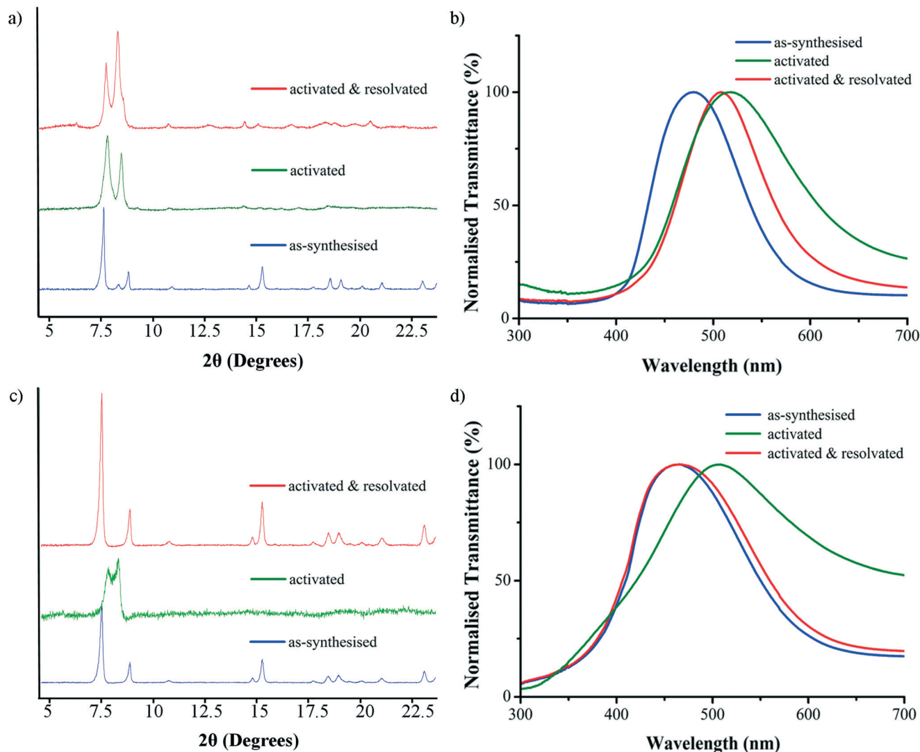
Fig. 5 a) Powder X-ray diffraction patterns and b) solid-state UV/vis transmittance spectra of a methanol-exchanged sample of 1-S (blue), 1 (green) and 1 -methanol obtained by resolution of an activated sample of 1 in methanol overnight (red), c) powder X-ray diffraction patterns and d) solid state UV/vis transmittance spectra of a methanol-exchanged sample of 1 -S (blue), 1 -S (green) and 1 -methanol obtained by resolution of an activated sample of 1 in methanol overnight (red). In the PXRD plots the peaks at ca. 2\theta = 7.5^\circ and 2\theta = 8.5^\circ correspond to 011 and 020 planes respectively which reflect the breathing of the MOF. In the sample of 1-S (blue) the peak at ca. 2\theta = 8.0^\circ corresponds to a small amount of the dried sample which forms as the material is packed into the capillaries.
