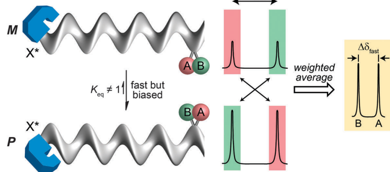
Fig. 5 Detection of screw-sense preference by NMR in the fast exchange regime. (a and b) Coalescence between signals in an equally populated pair of enantiomeric conformers; (c and d) coalescence between signals in an unequally populated pair of diastereoisomeric conformers.
