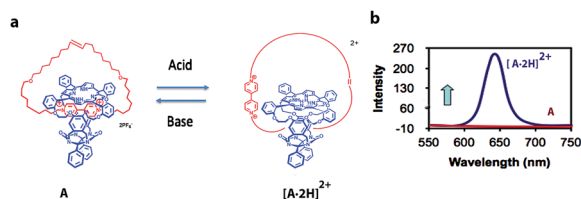
Fig. 2 (a) Acid-driven switching of porphyrin[2]catenane A . 21 (b) Fluorescence spectra of [2]catenanes A (red) and [\mathbf{A} \cdot 2\mathbf{H}]^{2+} (blue).
