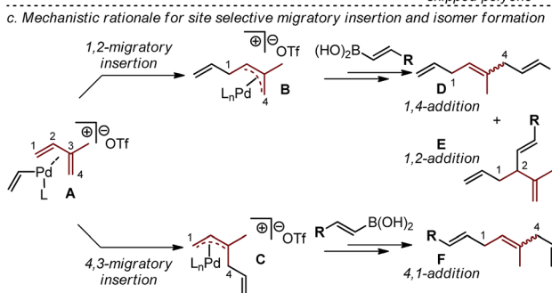
Fig. 1 Proposed 1,4-difunctionalization of isoprene and rationale accounting for regioisomers.
