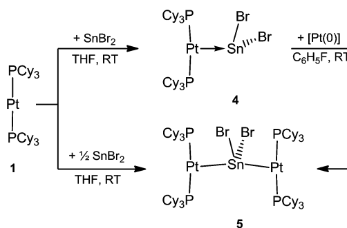
Scheme 2 Formation of the stannylene complexes 4 and 5 .
