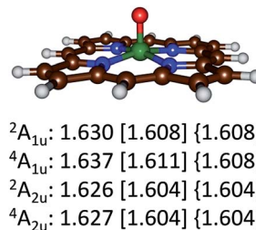
Fig. 4 Optimized geometries of the ^4,^2A_{2u} and ^4,^2A_{1u} states of ^4,^2A as calculated with UB3LYP/BS1 [UB3LYP/BS2] {UB3LYP-D3/BS2} with Fe–O bond lengths in angstroms.
