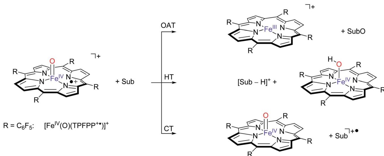
Scheme 3 Pathways observed for the reaction of [\text{Fe}^{\text{IV}}(\text{O})(\text{TPFP}^{++})]^+ ions (R = C 6 F 5 ) with selected substrates (Sub) as studied with FT-ICR MS.
