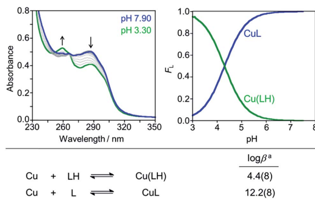
Fig. 3 Solution speciation of the \text{Cu(II)} – PyBD complex. Left: UV-vis spectra in the range of pH 3–8 ( [\text{Cu(II)}]/[\text{PyBD}] = 1 : 1; [\text{Cu(II)}]_{\text{total}} = 50 \mu M). Right: solution speciation diagram ( F_{\text{Cu}} = fraction of free Cu and Cu complexes). Bottom: stability constants of the \text{Cu(II)} – PyBD complex with charges admitted for clarity. Titrations were performed at room temperature with I = 0.1 M NaCl. a Error in the last digit is indicated in parentheses.
