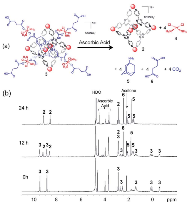
Fig. 2 (a) Chemical representation of the reduction of 3 by ascorbic acid and (b) ^1H NMR (400 MHz, R.T.) spectra showing reduction of 3 ( 0.8 mM) by ascorbic acid ( 8 mM) in deuterated PBS over 24 h at 37 °C.
