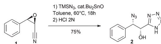
Scheme 1 Bu 2 SnO-catalyzed reaction of epoxynitrile 1 with TMSN 3 leads regioselectively to \alpha -hydroxy \beta -azido tetrazole 2 .
