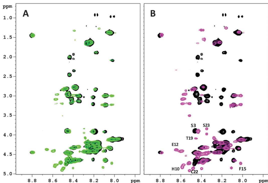
Fig. 8 2\text{D } ^1\text{H}-^1\text{H} TOCSY spectra (NH-H \alpha region) of Bri2-23 0.5 mM in \text{H}_2\text{O}:\text{D}_2\text{O} 90:10 at 298 K and pH 3.0 in the presence of (A) 0.5 equivalents of Hg(II) ions; (B) 0.7 equivalents of Hg(II) ions.
