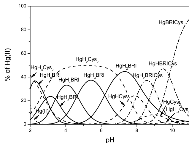
Fig. 5 Species distribution diagram for Hg(II) complexes of the Bri2-23 peptide in the presence of Cys at a 1:1:1 Hg/Bri2-23/Cys ratio; T = 298.2 K and I = 0.1 M in NaCl; C_{\text{Bri2-23}} = 5 \times 10^{-4} , C_{\text{Cys}} = 5 \times 10^{-4} , C_{\text{Hg(II)}} = 5 \times 10^{-4} .
