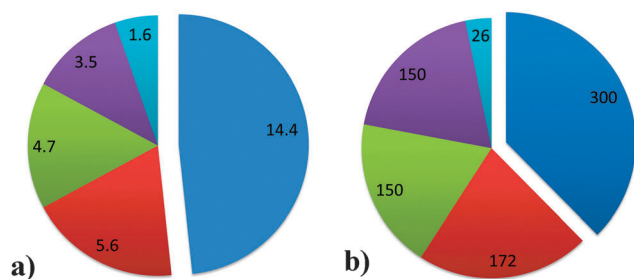
Fig. 1 (a) Installed capacities for the major conversion processes in refineries worldwide, in million barrels per day. (b) Number of refineries in which major conversion processes are installed. Refineries can have more than one technology installed. Data as of 2013, from ref. 1. Color-coding: fluid catalytic cracking (FCC): blue; hydrocracking: red; coking: green; thermal operations: purple; and resid hydrotreating: light blue.
