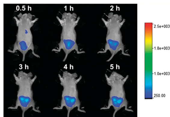
Fig. 65 Top: NIR emissive cyclen dosimeter 68 by Deng and Huang. Bottom: representative fluorescence images of mice (pseudocolour) that were injected with 68-Cu(II) (40 \mu\text{m} ), followed by \text{Na}_2\text{S} . The images were recorded after the injection of \text{Na}_2\text{S} within 5 h. Image reproduced with permission. 238
