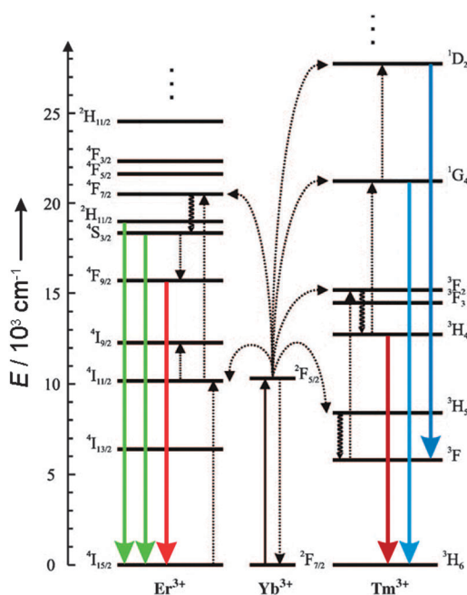
Fig. 1 Energy-level diagram of anti-Stokes processes in UCNPs ( \text{NaYF}_4 : \text{Yb} , \text{Er} / \text{Tm} ). The sensitizer ion \text{Yb}^{3+} absorbs NIR light, and the activator ions \text{Er}^{3+} or \text{Tm}^{3+} emit visible or NIR light. Sensitizer and activator ions are embedded in a hexagonal nanocrystal of \text{NaYF}_4 . Full arrows: radiative transitions, dotted arrows: non-radiative energy transfer, curled arrows: multiphonon relaxation. Adapted from ref. 2 with permission.
