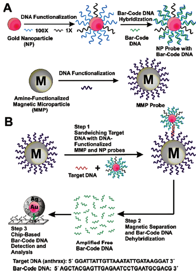
Fig. 8 Schematic illustration of the DNA-Bio-bar-code based ultrasensitive assay for DNA detection. (A) The preparation of the DNA modified Au NP and magnetic microparticle probes. (B) Schematics of the nanoparticle-based PCR-free DNA amplification and detection scheme. Reprinted with permission from ref. 80, copyright©2004, American Chemical Society.
