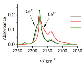
Fig. 4 IR spectra of CO adsorbed at -100 °C on activation, reduced by CO reaction and oxidized Ce-MCM-22-IEZ.
