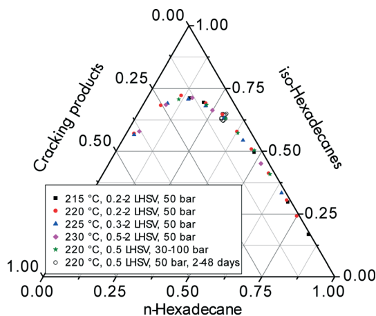
Fig. 7 Ternary plot of n -hexadecane, isohexadecanes and cracking product fractions for hydroisomerization over Pt-Pd/H-beta ( n_{\text{Si}}/n_{\text{Al}} = 25 ) by varying reaction conditions including temperature, space velocity, pressure, and time on-stream.
