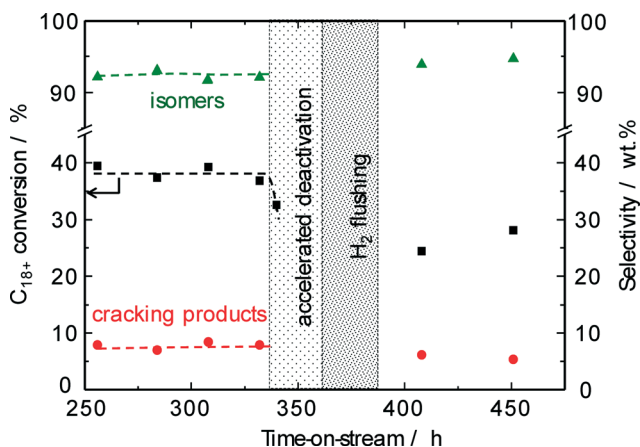
Fig. 10 Conversions of n -C 18+ paraffin feed and product selectivities as a function of time on-stream over Pd-Pt/H-beta ( n_{\text{Si}}/n_{\text{Al}} = 25 ) at 220 °C and 50 bar (LHSV = 0.5 h -1 ). The effect of hydrogen flushing after accelerated carbon deposition shows a marked reduction of the n_{\text{H}_2}/n_{\text{hydrocarbons}} ratio.
