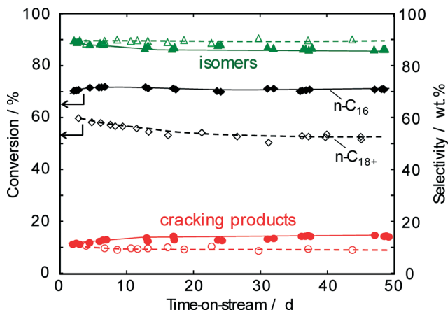
Fig. 9 Conversions of n -hexadecane (solid symbols) and n -C 18+ paraffin feed (open symbols) as well as product selectivities as a function of time on-stream over Pd-Pt/H-beta ( n_{\text{Si}}/n_{\text{Al}} = 25 ) at 220 °C and 50 bar (LHSV = 0.5 h -1 ).
