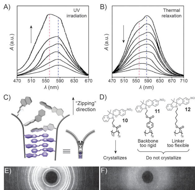
Fig. 7 Spectroscopic and structural evidence for MC stack formation. (A) SP \rightarrow MC isomerisation accompanied by MC aggregation during UV irradiation of a spiropyran-functionalised polymer 10 . (B) Thermal relaxation of the sample obtained in (A). (C) Schematic representation of "zipper crystallisation". (D) Structural formulas of spiropyran-functionalised polymers 10–12 differing in their crystallisation behaviour. (E) X-ray powder diffraction pattern of 10 . (F) X-ray powder diffraction pattern of 11 . [Adapted with permission from ref. 100 (Copyright 1984 American Chemical Society) (A and B) and ref. 107 (Copyright 1984 American Chemical Society) (E and F).]
