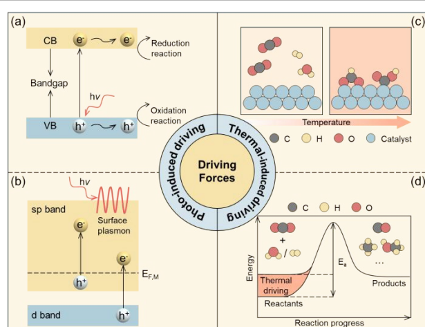
Fig. 2 Driving forces of photothermal CO 2 reduction: (a) photogenerated carriers, (b) plasmon-induced hot carriers, (c) thermal-driving intermolecular collisions and (d) thermal-induced increase in the population of electronic states, where E_{F,M} denotes Fermi level.
