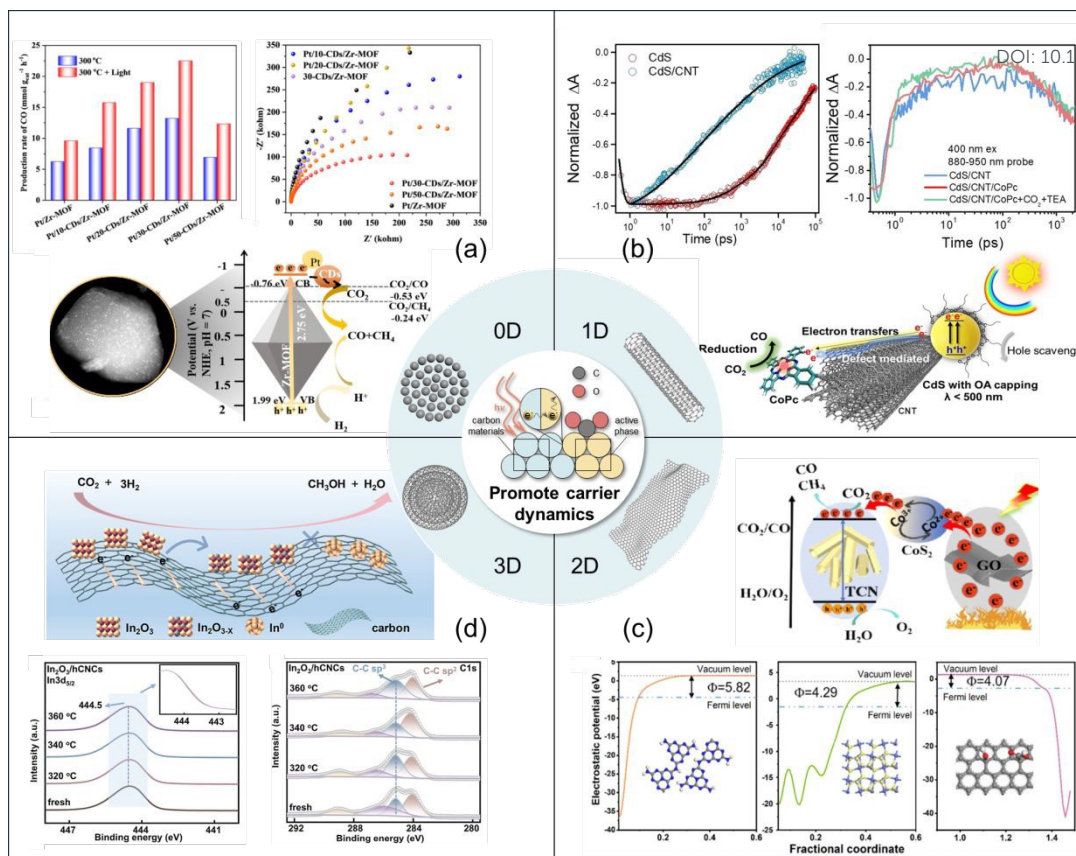
Fig. 5 Carbon-based functional phases for promoting the electron generation and transfer of carriers: (a) Effect of CDs content on carrier generation and transfer efficiency in Pt/CDs/Zr-MOF. Reproduced with permission. 32 Copyright 2025, Elsevier. (b) Effect of CNTs on carrier separation and transfer in CdS/CNT/CoPc. Reproduced with permission. 33 Copyright 2023, John Wiley & Sons. (c) Effect of graphene on carrier generation in GO/CoS 2 /TCN. Reproduced with permission. 99 Copyright 2025, Elsevier. (d) Effect of hCNCs on carrier transfer in In 2 O 3 /hCNCs. Reproduced with permission. 72 Copyright 2025, American Chemical Society.
