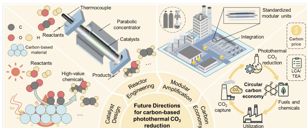
Fig. 12 Future directions of carbon-based photothermal CO 2 reduction.
