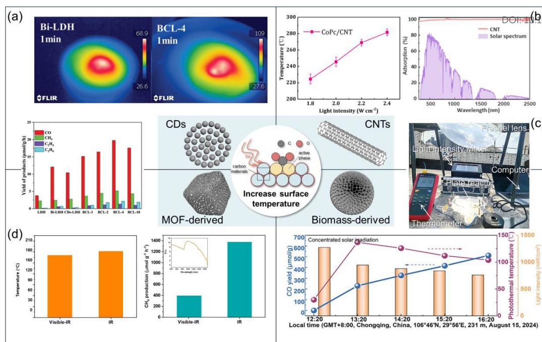
Fig. 6 Carbon-based functional phases for enhancing photo-induced heat effect: (a) Effect of CDs on surface catalytic temperature in Bi-CDs/LDH. Reproduced with permission. 98 Copyright 2024, John Wiley & Sons. (b) Effect of CNTs on surface catalytic temperature in CoPc/CNT. Reproduced with permission. 30 Copyright 2024, John Wiley & Sons. (c) Surface catalytic temperature of Bi 2 MoO 6 /BCF in outdoor experiments under natural light with a condenser. Reproduced with permission. 87 Copyright 2025, John Wiley & Sons. (d) The contributions of visible and infrared light in photothermal CO 2 methanation over Ni@C. Reproduced with permission. 109 Copyright 2021, John Wiley & Sons.
