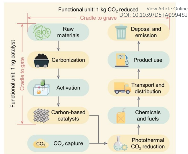
Fig. 11 General system boundary for carbon-based photothermal CO 2 reduction.
