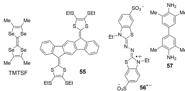
Fig. 18 Structures of TTF analogues and derivatives.
