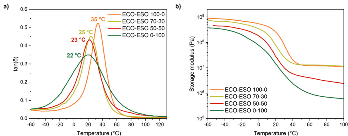
Fig. 5 Tan \delta vs. temperature curves (a) and storage modulus vs. temperature curves (b) for all UV-cured formulations.
