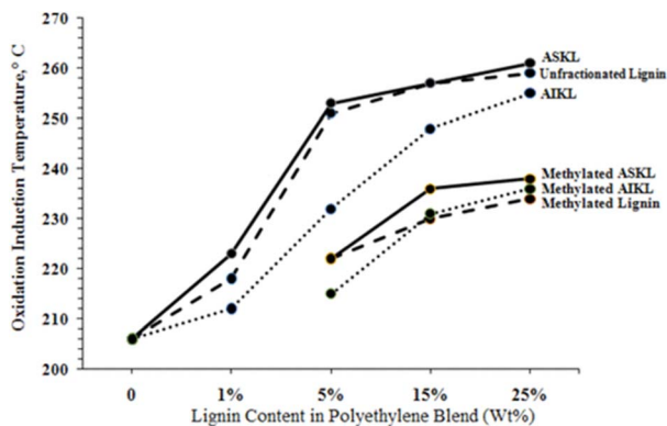
Fig. 14 Correlation of lignin content (unfractionated SKL and its fractions) in PE-blends with Ol_{temp} . Reproduced from ref. 168 with permission from the American Chemical Society, copyright 2015.
