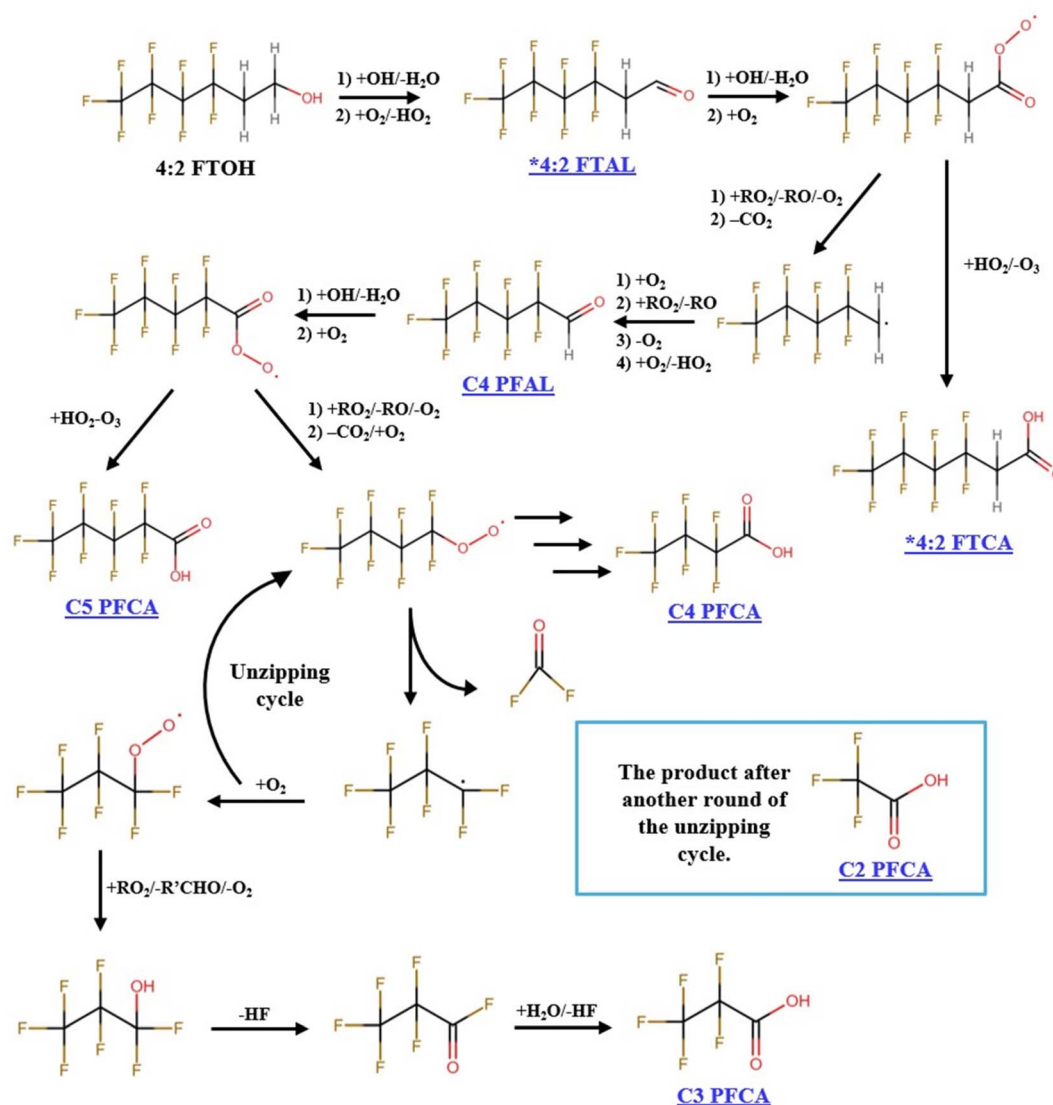
Fig. 1 The proposed atmospheric degradation mechanism of the 4:2 FTOH + \cdot\text{OH} radicals in a NO x -free environment. 18 The expected stable end products are underlined in blue, with the specific products observed in this work being asterisked. The compounds shown are as follows: 4:2 fluorotelomer aldehyde (4:2 FTAL); 4:2 fluorotelomer carboxylic acid (4:2 FTCA); perfluoropentanal (C 4 PFAL); perfluoropentanoic acid (C 5 PFCA); perfluorobutanoic acid (C 4 PFCA); pentafluoropropionic acid (C 3 PFCA); trifluoroacetic acid (C 2 PFCA).
