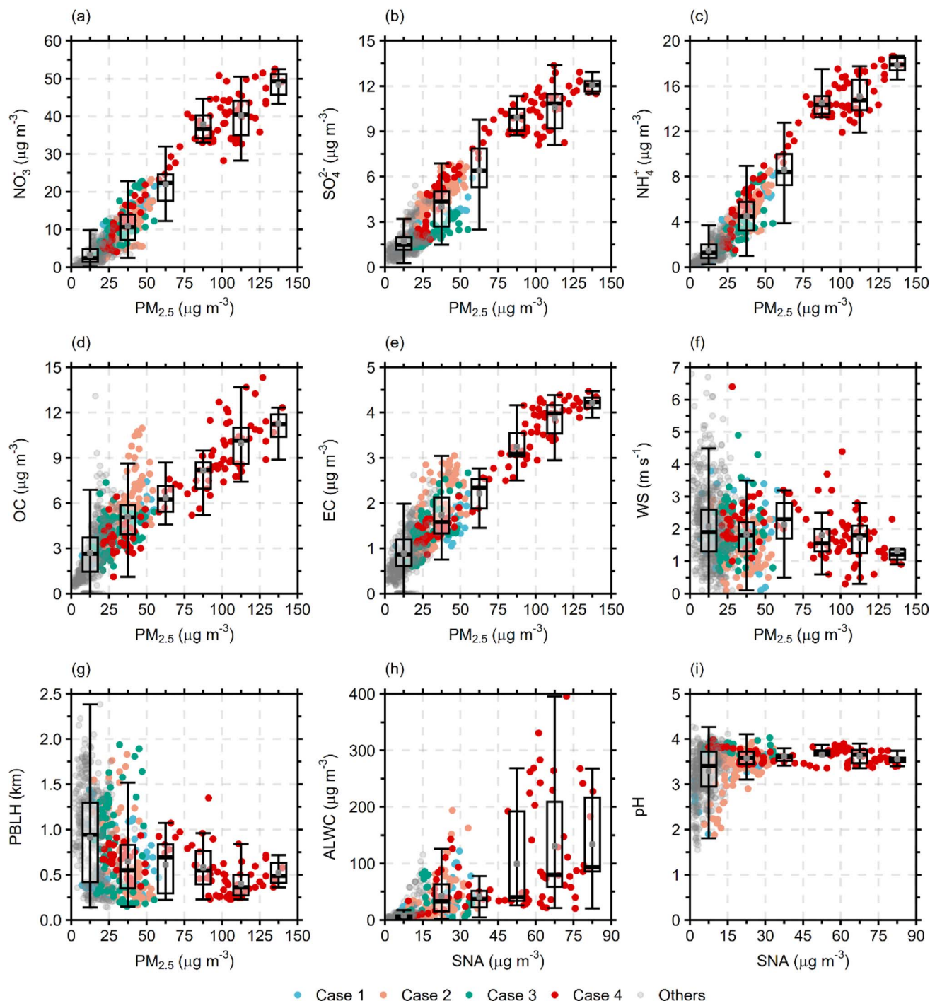
Fig. 1 Correlations of PM_{2.5} , its components and related variables during the measurement period. (a–e) Correlations between PM_{2.5} concentrations and major PM_{2.5} components. (f and g) Correlations with meteorological variables, including WS and PBLH. (h and i) Correlations between the sum of sulfate, nitrate and ammonium (SNA), ALWC and pH.
