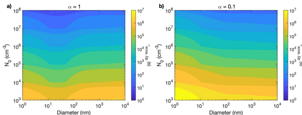
Fig. 1 Characteristic self-coagulation timescale ( \tau_{\text{scoa}} ) for monodispersed particles as a function of particle diameter ( D_p = 1 \text{ nm} - 10 \text{ }\mu\text{m} ) and particle number concentrations ( N_0 = 10^3 - 10^8 \text{ cm}^{-3} ) with different coagulation efficiencies: (a) \alpha = 1 , (b) \alpha = 0.1 .
