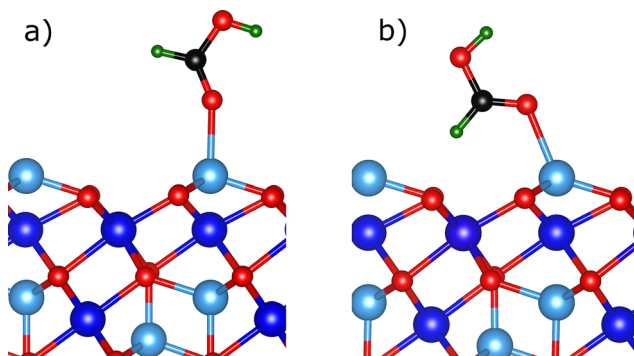
Fig. 9 Geometries for molecularly adsorbed formic acid on a tetrahedrally (tet1) terminated \text{Fe}_3\text{O}_4(111) surface. (a) Monodentate binding mode. (b) Quasi-bidentate binding mode.
