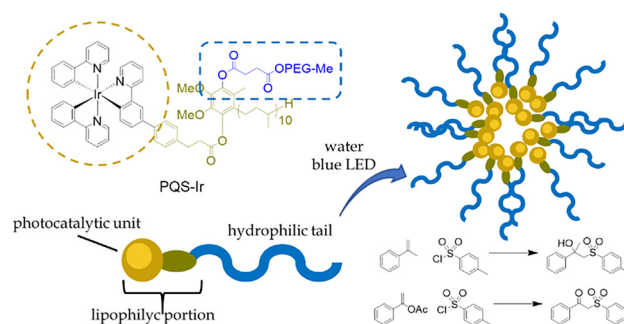
Fig. 9 Structure of the ubiquinol-based, amphoteric photocatalyst PQS-Ir and the schematic representation of the self-assembled micelles in water with reaction schemes of the \beta -hydroxylsulfonation of aromatic alkenes and the di-functionalization of aromatic enol acetates, enabled in water via micellar photocatalysis. 77
