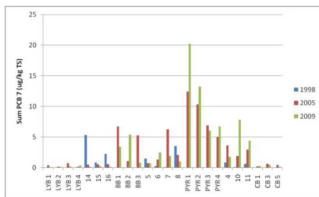
Figure 8. Concentrations in three years of the sum of 7 PCB congeners ( \Sigma_7\text{PCB} = PCB 28, 52, 101, 118, 138, 153, 180) in sediment from Isfjorden, Svalbard. Data from 1998 from 199 data from 2005 200 and data from 2009 201 . LYB1 – st. 16 = stations in Adventfjorden, BB1 – st. 8 = stations in Grøn fjorden, PYR1 – st. 11 = stations in Billefjorden, CB1 – CB5 = stations in Coles Bay, Figure reproduced with permission from 176 .
