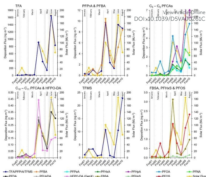
Figure 5: Deposition fluxes per precipitation event (ng m -2 ) of TFMS, PFHxS, PFOS, FBSA, HFPO-DA (GenX) and C 2 –C 11 PFCAs in surface snow on the Foxfonna ice cap during January to August 2019, plotted alongside the solar flux (MJ m -2 ). 174, 175 . Reproduced under the Creative Commons Attribution 4.0 International licence (CC BY 4.0).
