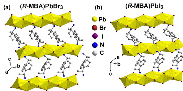
Fig. 1 Crystal structure diagrams of (a) (R-MBA)PbBr 3 and (b) (R-MBA)PbI 3 obtained from SCXRD data at 100 K. The structure comprises one-dimensional chains of lead-halide octahedra with R-MBA cations positioned between them.
