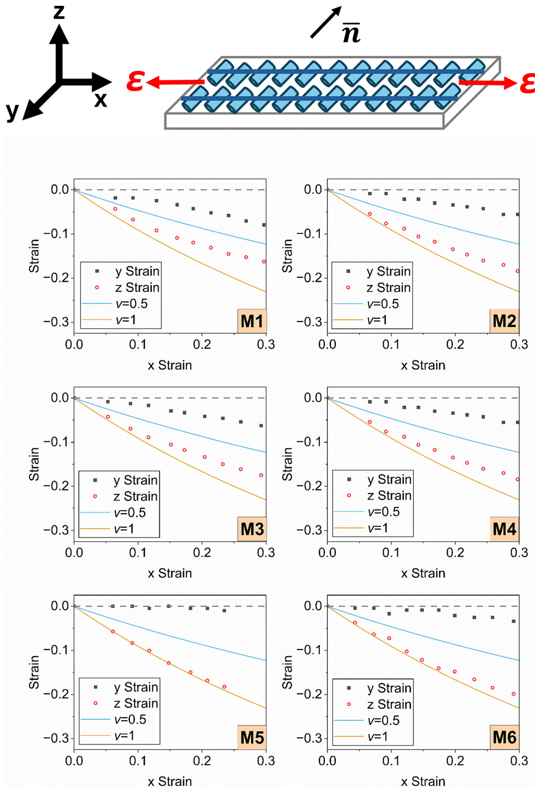
Fig. 5 The effect of an applied x-strain, perpendicular to the director, on the observed strain in the width (y-axis, black symbols) and thickness (z-axis, open red symbols) of planar aligned samples of each LCE. In all cases, strains are plotted as engineering strains. In all graphs, the blue and yellow lines display the strain behaviour expected for a system with a Poisson's ratio ( \nu ) of 0.5 (i.e. isotropic rubber behaviour) and 1 (incompressible layers) respectively, and the grey dashed lines represent \nu of 0. The schematic atop the figure displays the direction of applied strain ( \epsilon ) relative to the director/smectic layer normal ( \bar{n} ), with smectic layers being displayed as dark blue lines.
