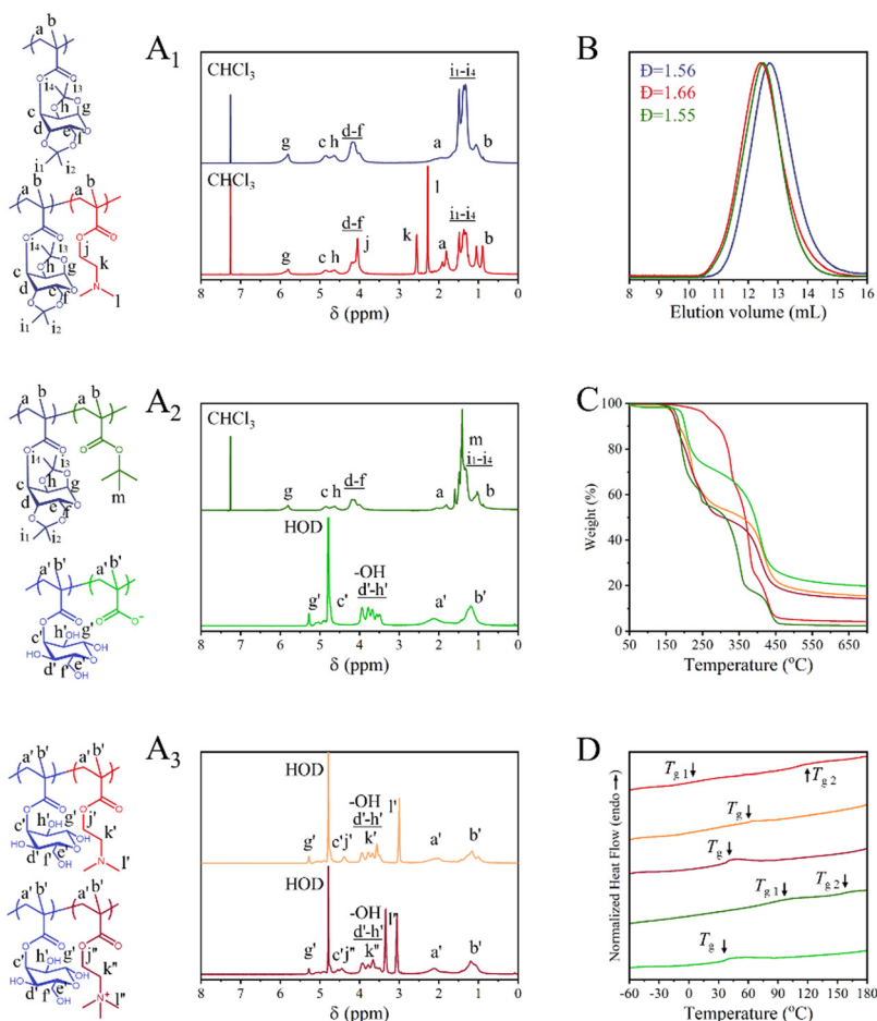
Fig. 1 Characterization of oppositely charged glycosylated block copolymers and their precursors. (A) 1 –(A) 3 1 H NMR spectra of the polymers: PPrGlcMA 72 (dark blue), PPrGlcMA 72 - b -PDMAEMA 71 (red), and PPrGlcMA 72 - b -PtBMA 85 (dark green), PGlcMA 72 - b -PMAA 85 (light green), PGlcMA 72 - b -PDMAEMA 71 (orange), PGlcMA 72 - b -PMETAL 71 (dark red). (B) SEC elugrams of PPrGlcMA 72 (dark blue), PPrGlcMA 72 - b -PDMAEMA 71 (red) and PPrGlcMA 72 - b -PtBMA 85 (dark green). (C) TGA and (D) DSC analyses of PPrGlcMA 72 - b -PDMAEMA 71 (red), PGlcMA 72 - b -PDMAEMA 71 (orange), PGlcMA 72 - b -PMETAL 71 (dark red), PPrGlcMA 72 - b -PtBMA 85 (dark green) and PGlcMA 72 - b -PMAA 85 (light green).
