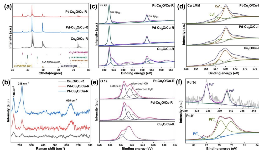
Fig. 2. (a) XRD patterns and (b) Raman spectra of Pt-Cu 2 O/ \text{Cu} -R, Pd-Cu 2 O/ \text{Cu} -R, and Cu 2 O/ \text{Cu} -R; XPS spectra of Pt-Cu 2 O/ \text{Cu} -R, Pd-Cu 2 O/ \text{Cu} -R, and Cu 2 O/ \text{Cu} -R: (c) Cu 2p; (d) AES spectra of Cu LMM; (e) O 1s and (f) Pd 3d and Pt 4f.
