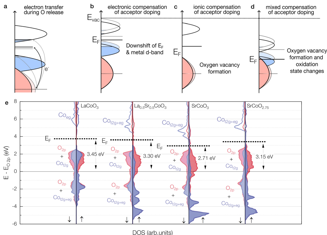
Fig. 3 (a) e^- Transfer from the O 2p band to E_F during oxygen release with the corresponding decrease of the projected density of oxygen states. (b–d) Simplified evolution of the electronic structure of a generic perovskite oxide upon (b) electronically, (c) ionically and (d) mixed electronically and ionically compensated acceptor doping. (e) Atom-projected densities of states for cobaltate perovskites with different A-site cations and V_O^\bullet concentrations. Gradually replacing La with Sr in \text{La}_{1-x}\text{Sr}_x\text{CoO}_3 leads to a lower metal d-band and E_F . Introducing V_O^\bullet in \text{SrCoO}_{3-\delta} conversely leads to a higher metal d-band and E_F .
