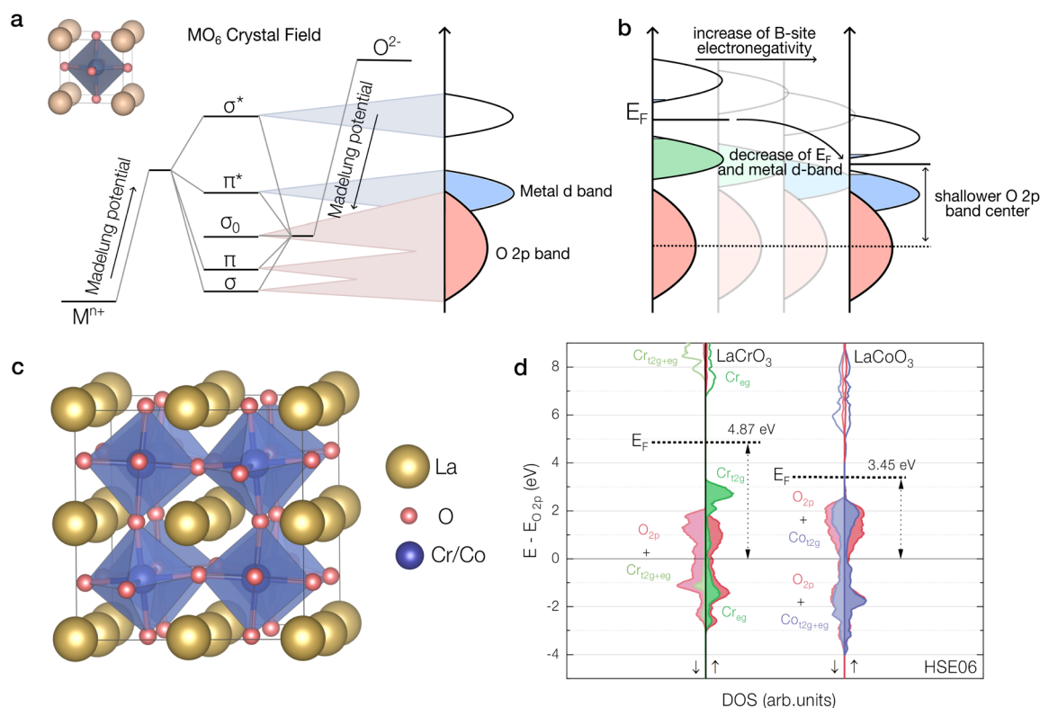
Fig. 2 (a) Simplified evolution of an exemplary transition metal perovskite oxide band structure from the molecular orbital diagram for octahedral \text{MO}_6 . (b) Qualitative change of the electronic structure with increasing B-site cation electronegativity. E_F and the metal d-band shift down, leading to a shallower O 2p band center. (c) Model of a 2 \times 2 \times 2 perovskite unit cell used for hybrid calculations (tilting angles slightly differ between \text{LaCoO}_3 and \text{LaCrO}_3 ). (d) Projected densities of states for \text{LaCrO}_3 and \text{LaCoO}_3 , with the energy of the respective centroid of the occupied O 2p states taken as the reference energy.
