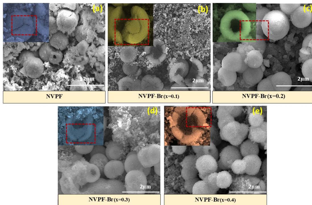
Fig. 5 Post-cycling SEM image of cathode surfaces. Surface morphologies of cathodes after cycling for pristine NVFP and Br-substituted samples: (a) NVFP, (b) NVFP-Br ( x = 0.1 ), (c) NVFP-Br ( x = 0.2 ), (d) NVFP-Br ( x = 0.3 ), and (e) NVFP-Br ( x = 0.4 ) [magnification 45 000 \times , scale bar indicates 2 \mu\text{m} length]. Insets show corresponding high-magnification images of the surface features [magnification 115 000 \times ].
