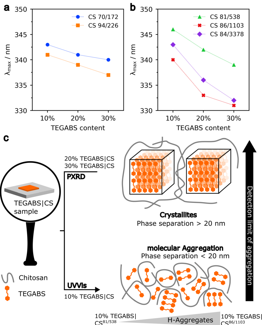
Fig. 6 UV-Vis characterization of native TEGABS|CS thin films. (a and b) UV-Vis spectra showing the wavelength \lambda_{\max} of the \pi-\pi^* transitions of the TEGABS|CS films. (c) Indicates the two kinds of aggregates detectable via PXRD and UV-Vis spectroscopy. It has also been demonstrated that UV-Vis can be used to qualitatively differentiate the proportion of H-aggregates present in 10% TEGABS|CS films.
