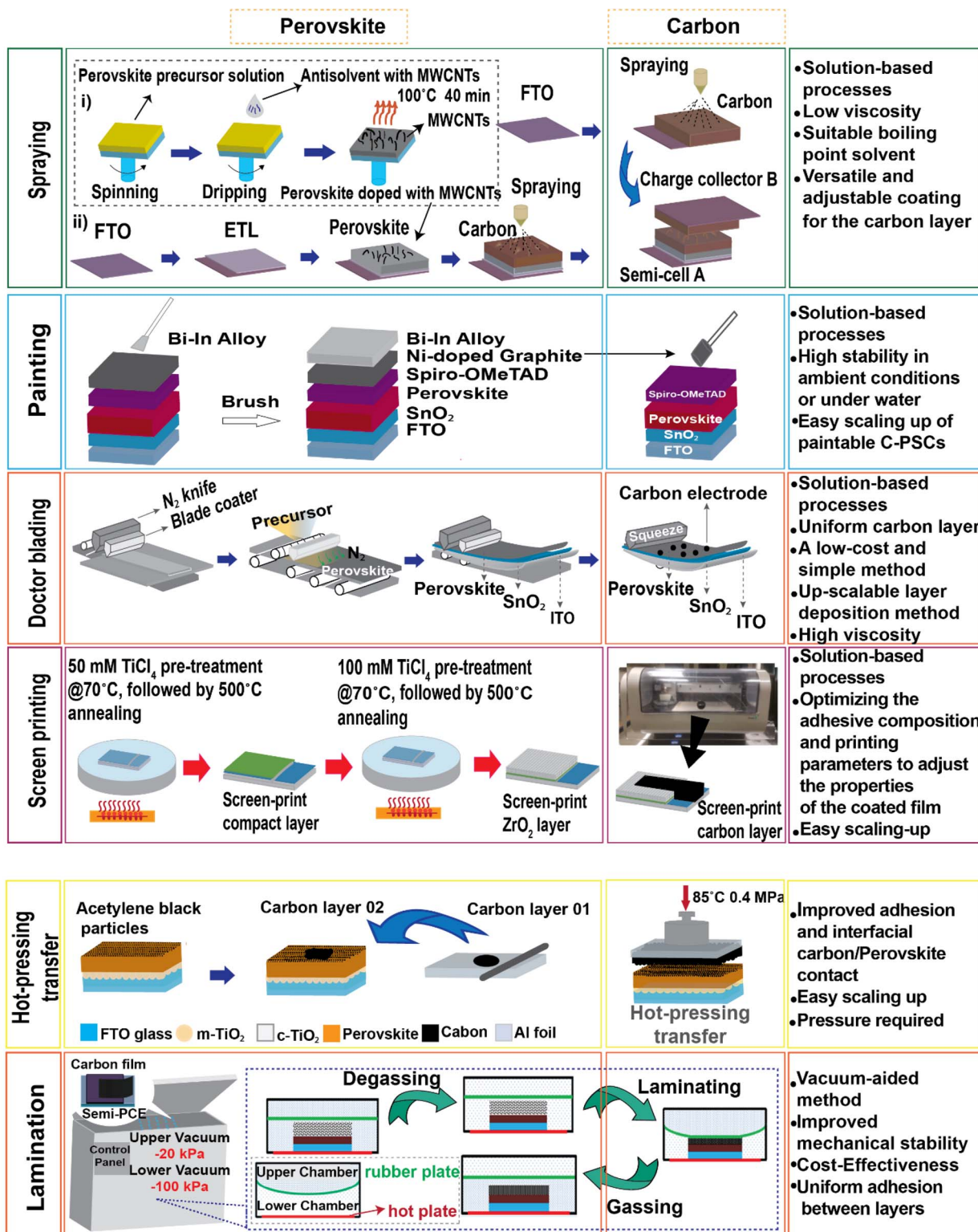
Fig. 3 Schematic illustration of the structure of large-area C-PSCs and their fabrication methods.
