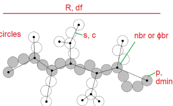
Fig. 7 2D schematic of an aggregate showing d_p = diameter of primary particles; R = end-to-end distance/aggregate size; c = connectivity (branching), 3 > c \geq 1 for aggregates; d_{\min} = tortuosity of aggregates independent of c , 3 > d_{\min} \geq 1 ; d_f = mass fractal dimension d_f = c \times d_{\min} , 3 > d_f \geq 1 reflecting packing density; z = degree of aggregation = (R/d_p)^{d_f} ; p = minimum (short-circuit) path, grey circles p = (R/d_p)^{d_{\min}} ; s = connective path, black lines s = (R/d_p)^c .
