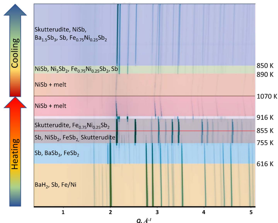
Fig. 2 High-temperature in situ powder X-ray diffraction data obtained upon heating to 1070 K and subsequent cooling of a \text{BaH}_2 , Sb, Fe, Ni precursors mixture. Data represented as a contour plot, and each horizontal section corresponds to a PXRD pattern where darker shading indicates higher relative diffraction intensity. The temperature ranges with distinct crystalline phases present are highlighted in yellow, light blue, grey, pink, orange, light green, and blue.
