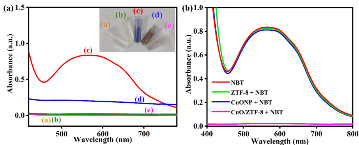
Fig. 3 Absorbance spectra of (a) \text{O}_2^{\cdot-} in DMSO (orange), (b) 1 \text{ mg mL}^{-1} of NBT in 0.1 M PBS (pH 7) (green), (c) \text{O}_2^{\cdot-} -NBT system (red), (d) 0.5 \text{ mg mL}^{-1} of CuO/ZTF-8 in 0.1 M PBS (pH 7) (blue), and (e) \text{O}_2^{\cdot-} -NBT system in the presence of CuO/ZTF-8 (pink). (Inset) Visual representation of the colour changes observed (b) \text{O}_2^{\cdot-} -NBT system in the absence (red) and presence of ZTF-8 (green), CuONP (blue), and CuO/ZTF-8 (pink) in 0.1 M PBS (pH 7).
